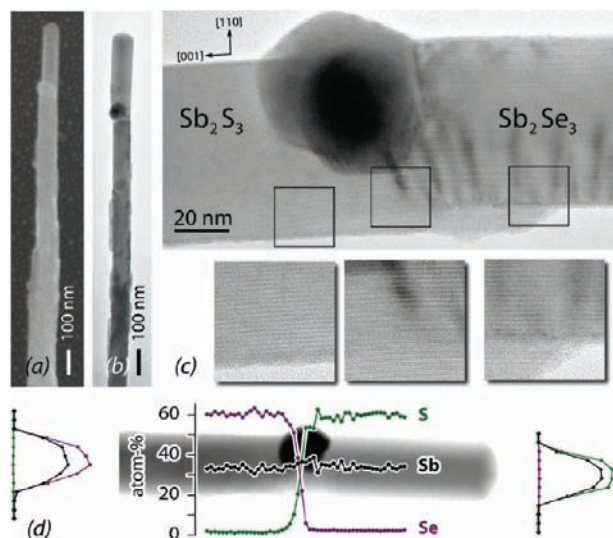
Figure 4. Perfectly anisotropic heteroepitaxial deposition of \text{Sb}_2\text{S}_3 onto \text{Sb}_2\text{Se}_3 wires at 160 °C. (a) SEM and (b) TEM images. (c) HRTEM images near the interface, in which no crystal defect is visible. (d) EDX linescans of the segmented wire. The radial scans show the absence of S (green) in the \text{Sb}_2\text{Se}_3 segment and of Se (purple) in \text{Sb}_2\text{S}_3 ; the axial scan, scaled to display the stoichiometry, shows an interface more abrupt than the EDX resolution.
