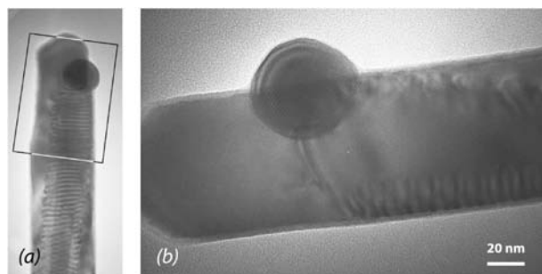
Figure 3. At 120 °C, conformal and anisotropic heteroepitaxial growths of \text{Sb}_2\text{S}_3 onto \text{Sb}_2\text{Se}_3 wires coexist, as shown by (a) TEM and (b) HRTEM images of one such structure. The region of (a) chosen for closer investigation in (b) is marked by a rectangle.
